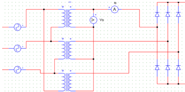
Figure 2. Simulation in psim
