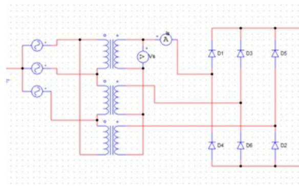
Figure 1: Three-Phase Rectifier Circuit
