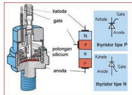
Figure 2. Thyristor
